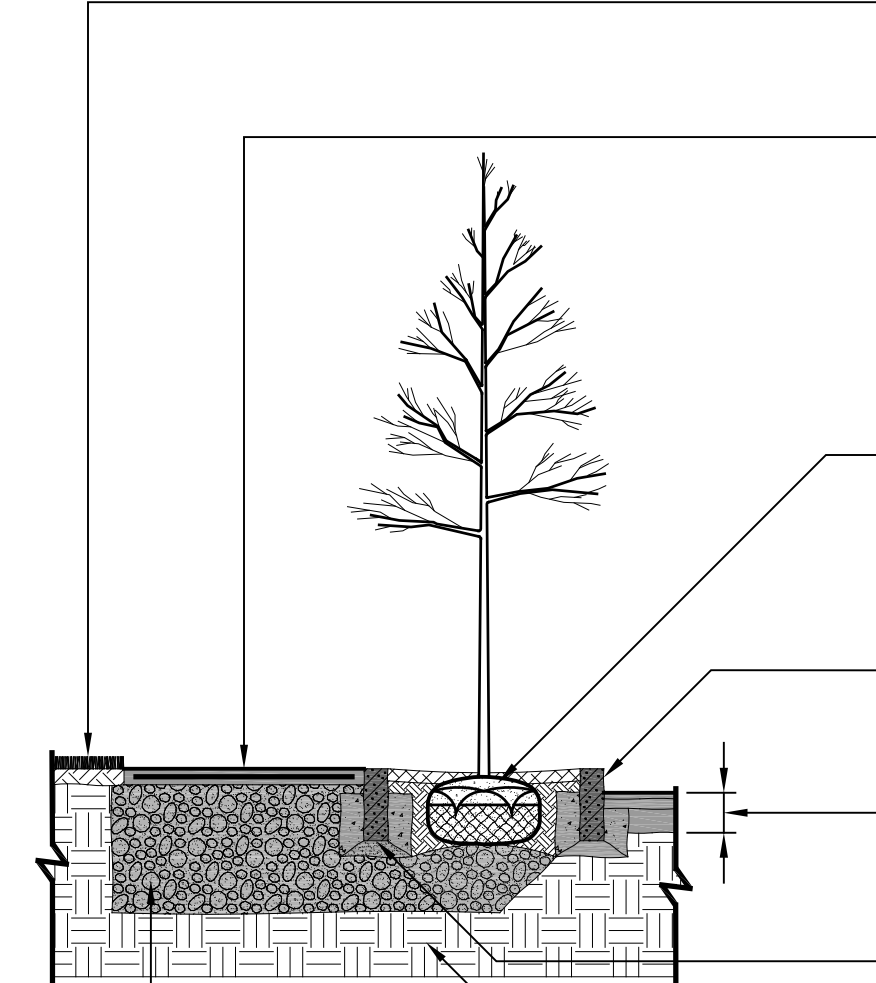
SECTION B-B
